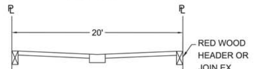
STANDARD CROSS-SECTION (PLAN VIEW)
