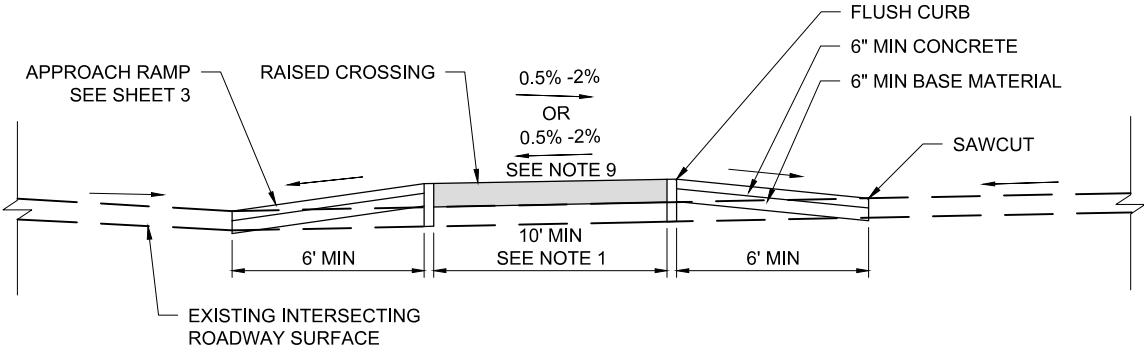
B CONCRETE RAMPS AND ASPHALT CROSSWALK 1,7 N.T.S.
