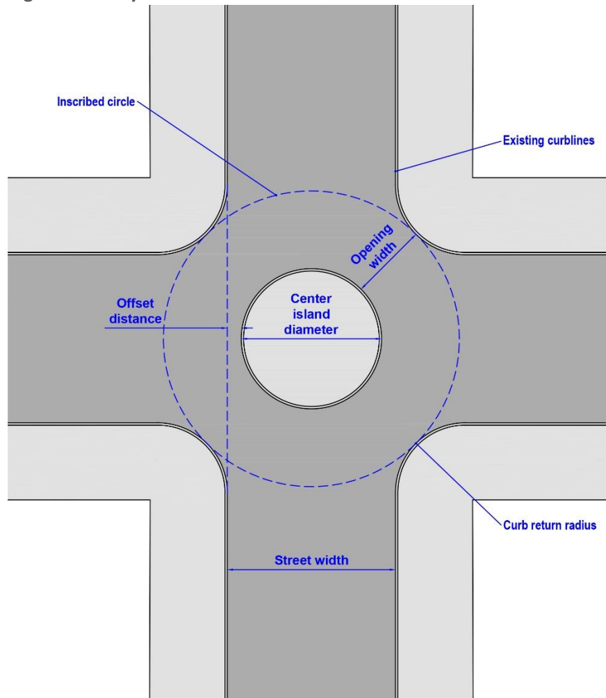
Figure 7-5 Key Geometric Elements
