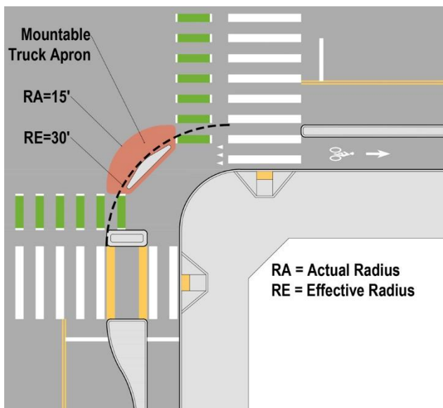
Figure 2-8 Type II One-Side Curb Extension with a Protected Bike Lane
