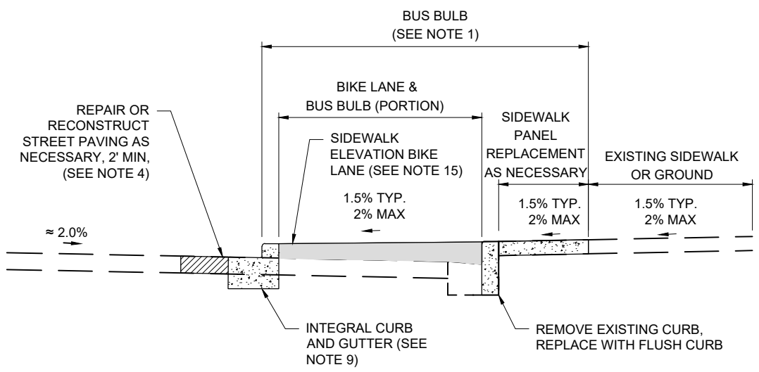
A 11 TYPICAL SECTIONS AT CONSTRAINED BUS BULB SHALLOW ROAD CROSS SLOPES
