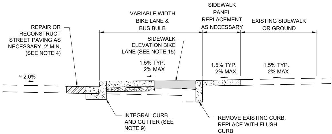
A 12 TYPICAL SECTIONS AT CONSTRAINED BUS BULB SHALLOW ROAD CROSS SLOPES
