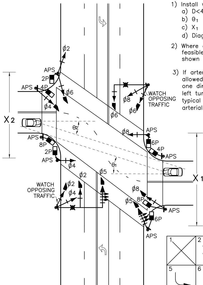
Right joggled Intersection Protected Left Turn
