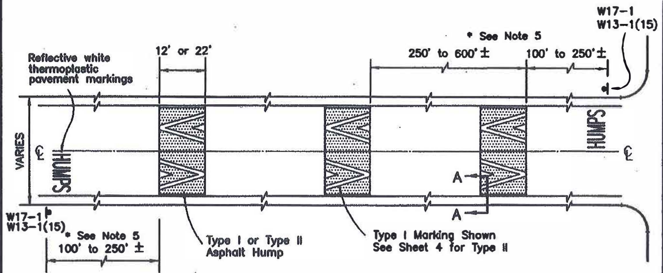
Layout on Two-Lane Street
