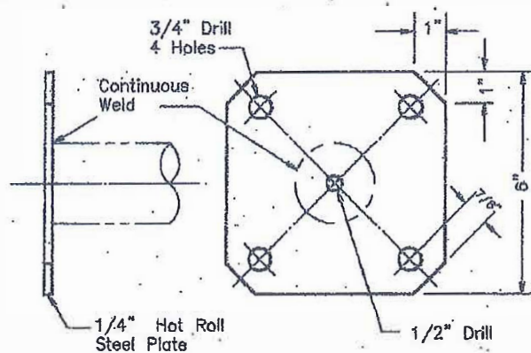
DETAIL: Post Flange Base
