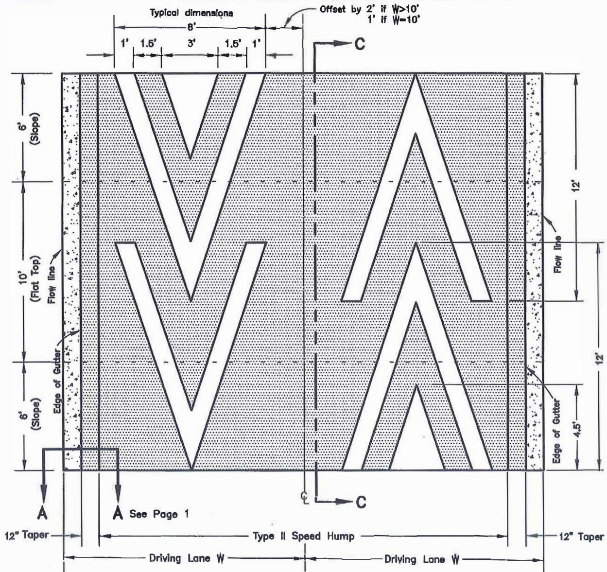
Type II Speed Hump Marking (Chevron II)
