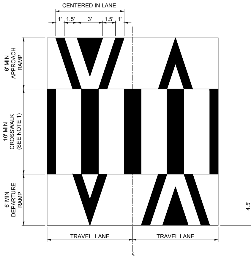
RAISED CROSSWALK MARKING (CHEVRON III)
