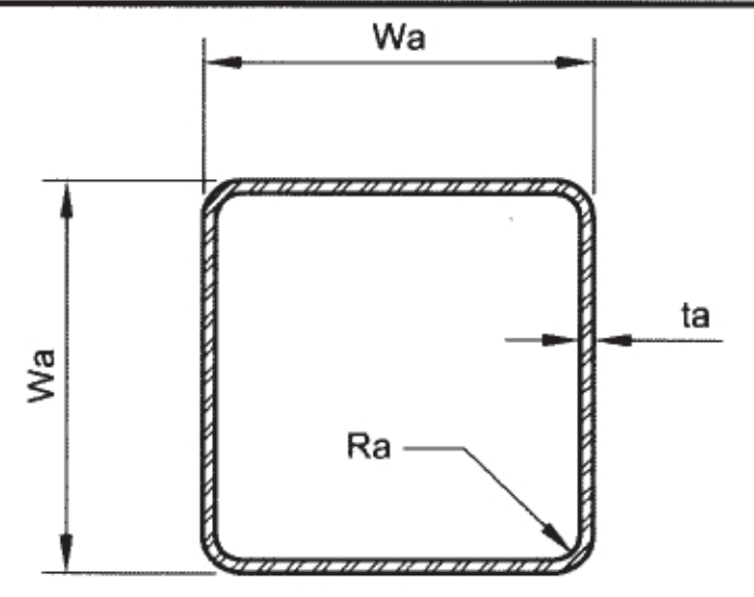
A8 TYP ARM SECTION SCALE : 3/4" = 1'-0" S-1
