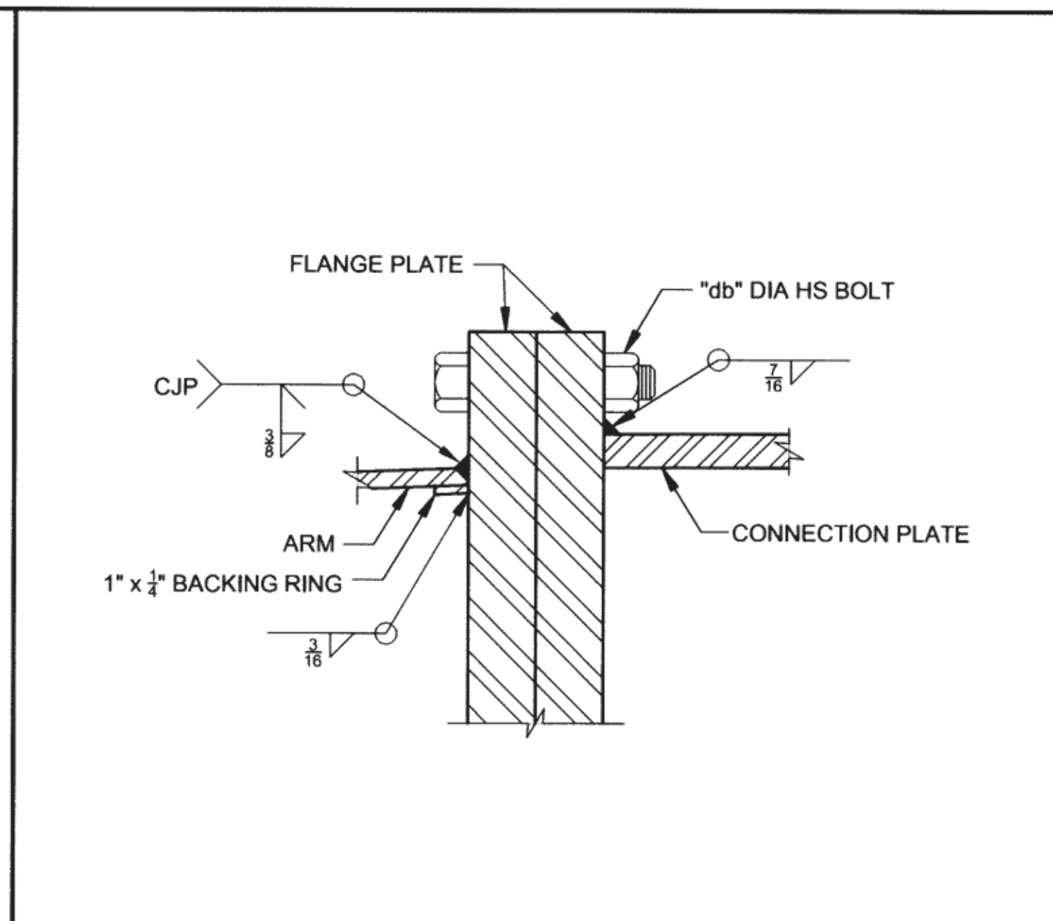
I5 FLANGE PLATE WELD DETAIL SCALE: NTS
