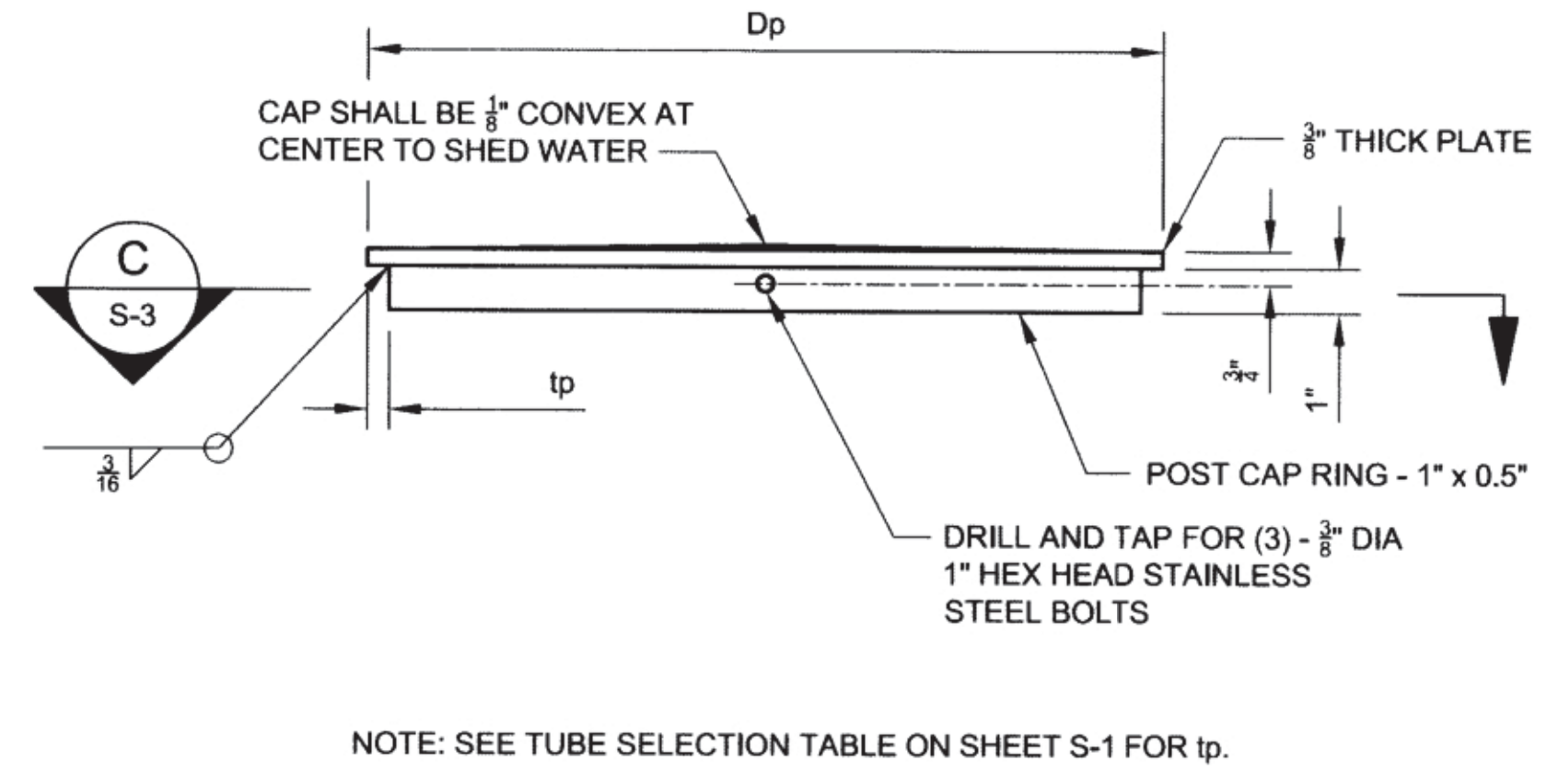
E7 POST CAP DETAIL SCALE: 3" = 1'-0"
