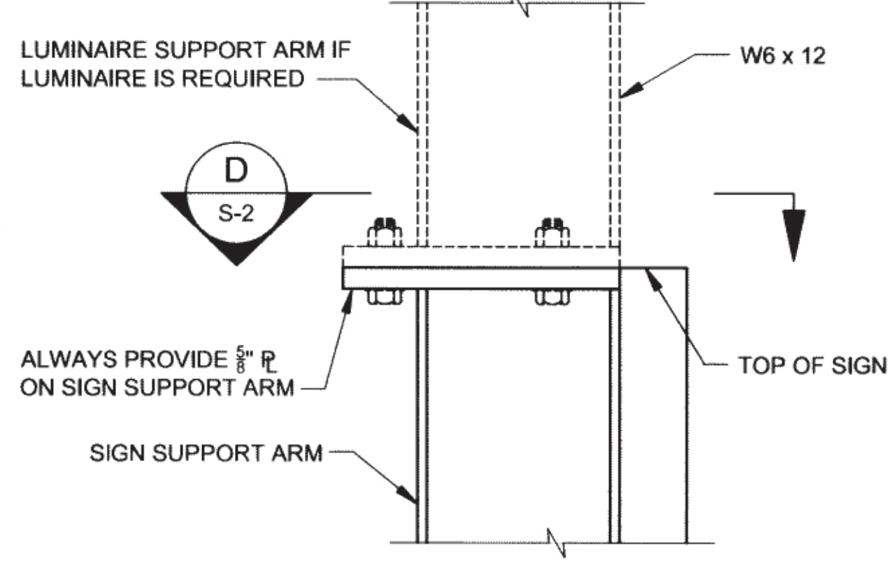
I10 ARM SPLICE DETAIL SCALE : 3" = 1'-0"
