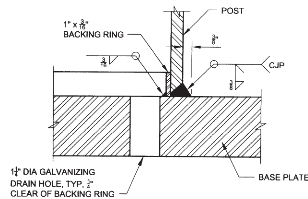
A1 POST TO BASE PLATE CONNECTION DETAIL SCALE : NTS S-4
