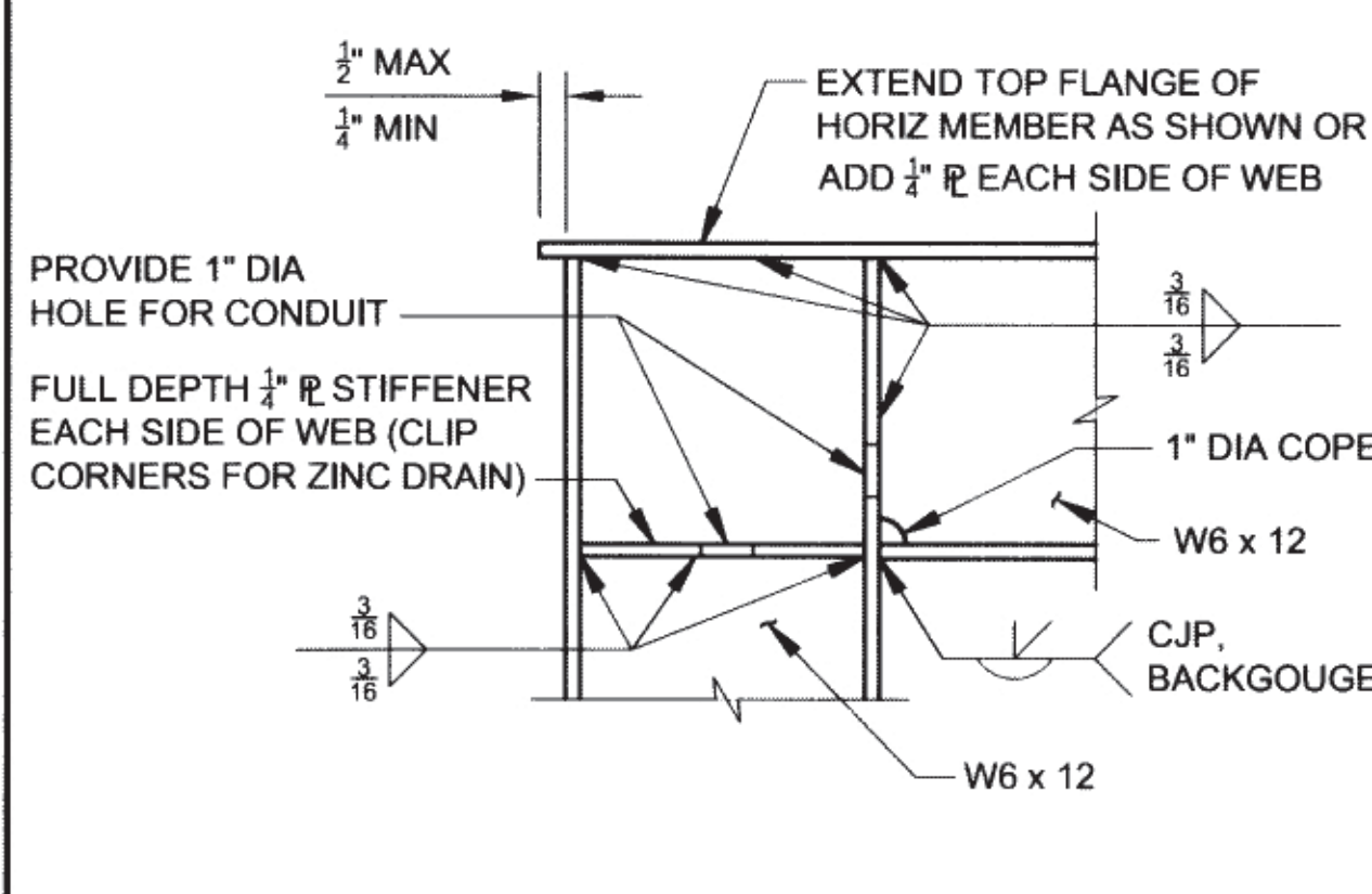
I7 CORNER DETAIL SCALE : 3" = 1'-0"
