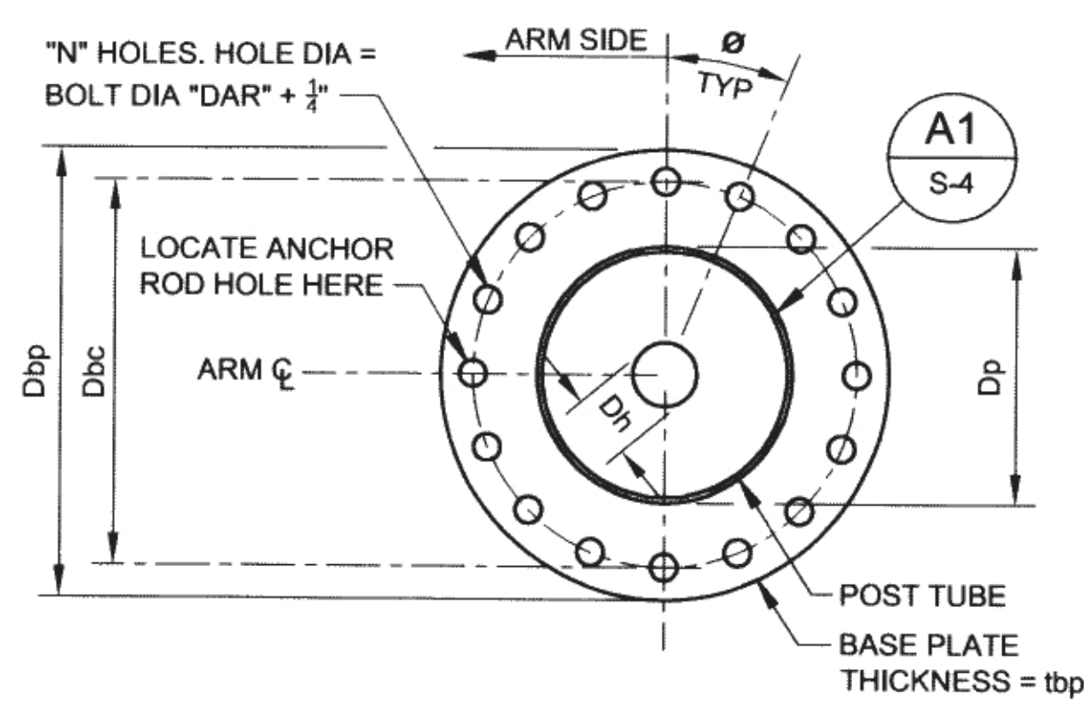
J6 BASE PLATE DETAILS SCALE : 3/4" = 1'-0" S-5
