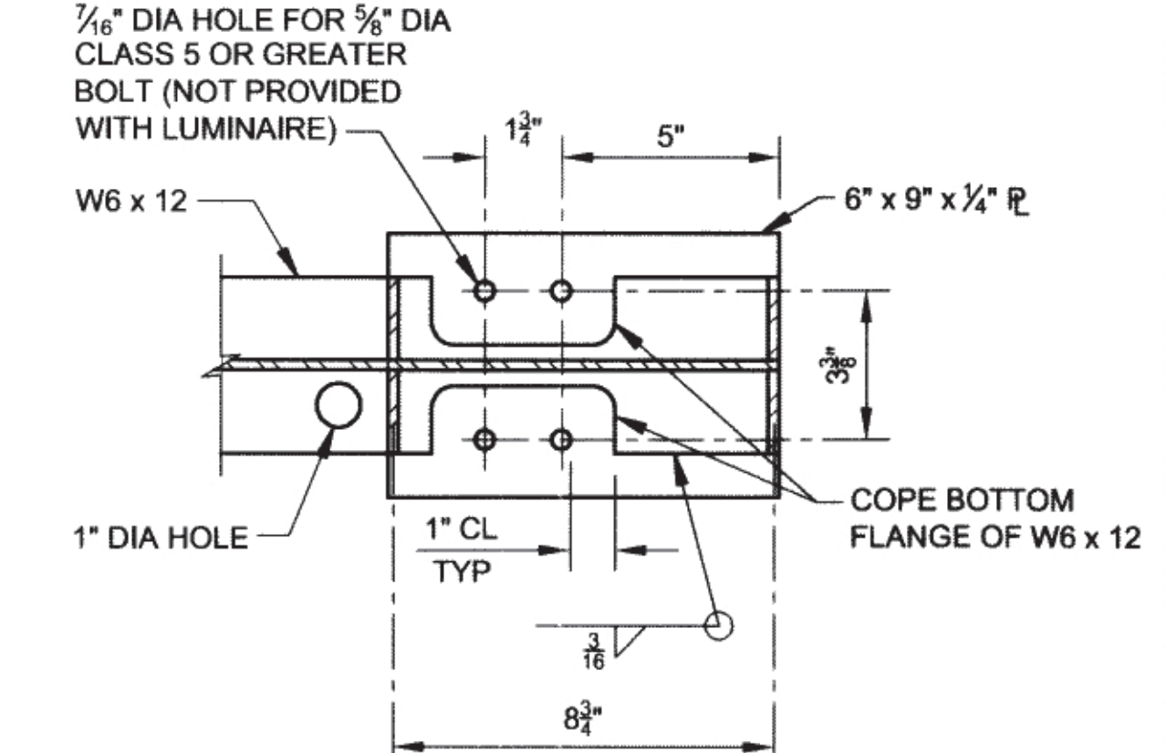
I14 SECTION B SCALE : 3" = 1'-0"
