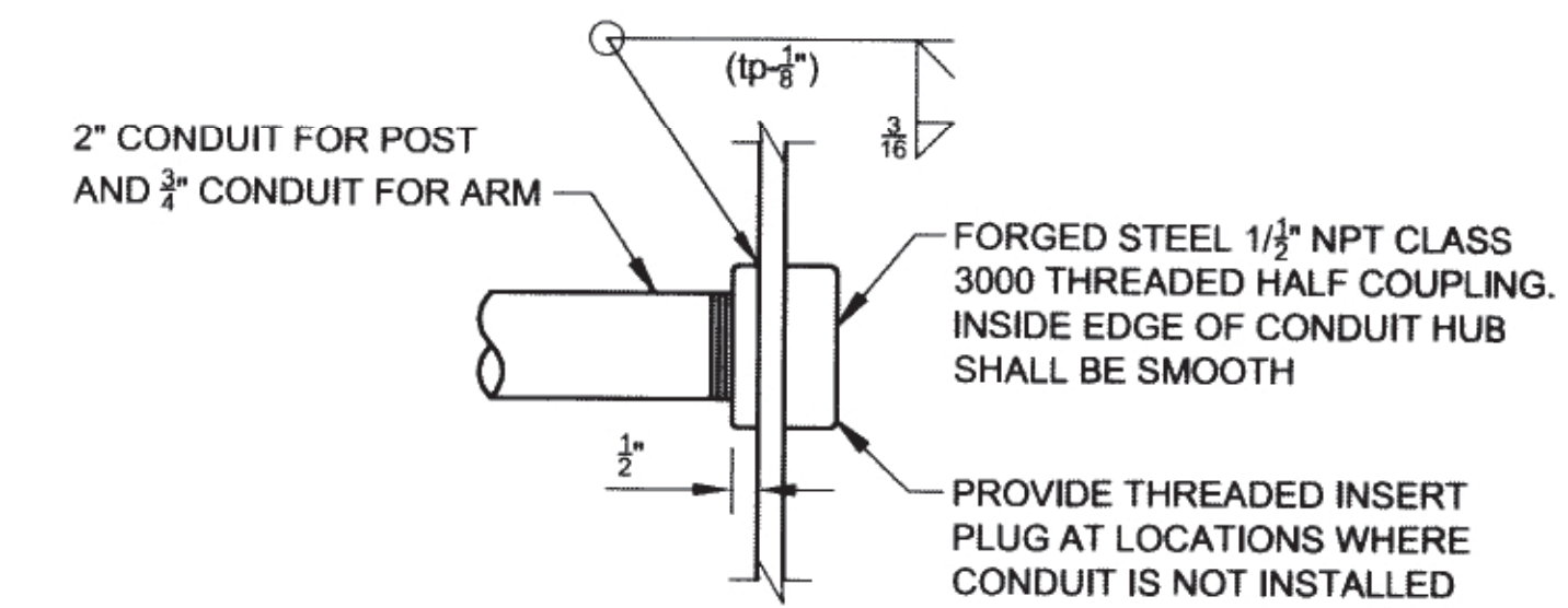
G11 HUB DETAIL SCALE : 3" = 1'-0" S-1
