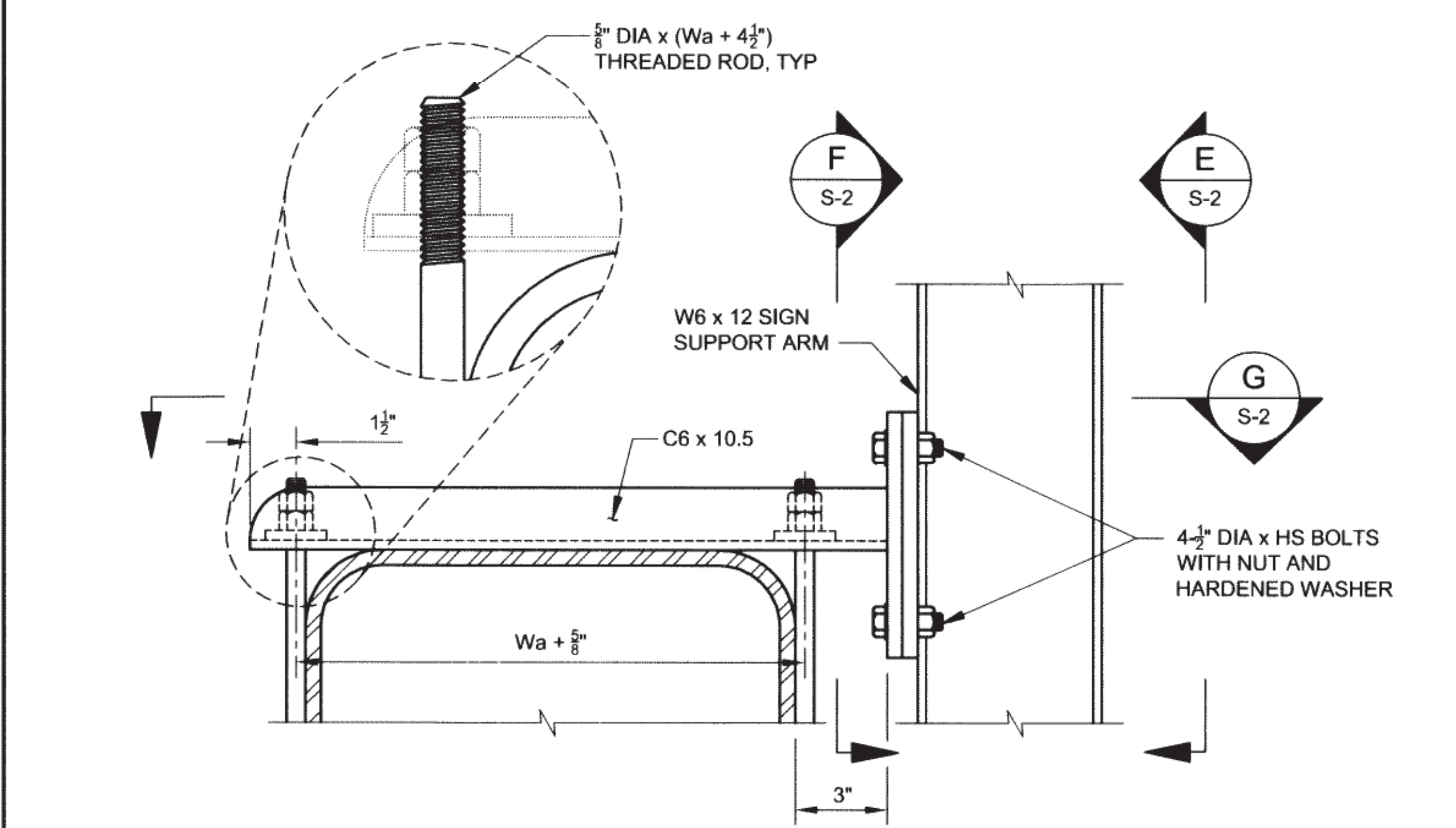
E7 CANTILEVER ARM CONNECTION SCALE : 3" = 1'-0"
