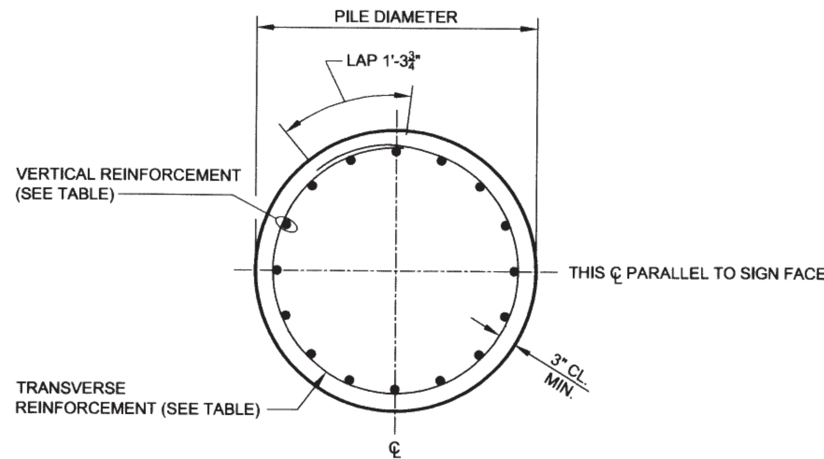
17 SECTION A SCALE : 3/4" - 1'-0" S-5
