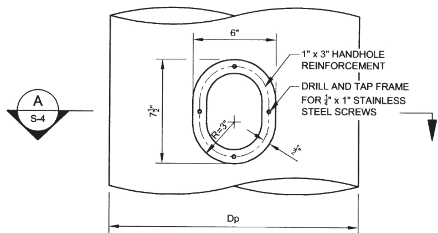
J1 HANDHOLE DETAILS SCALE : 3" = 1'-0" S-1
