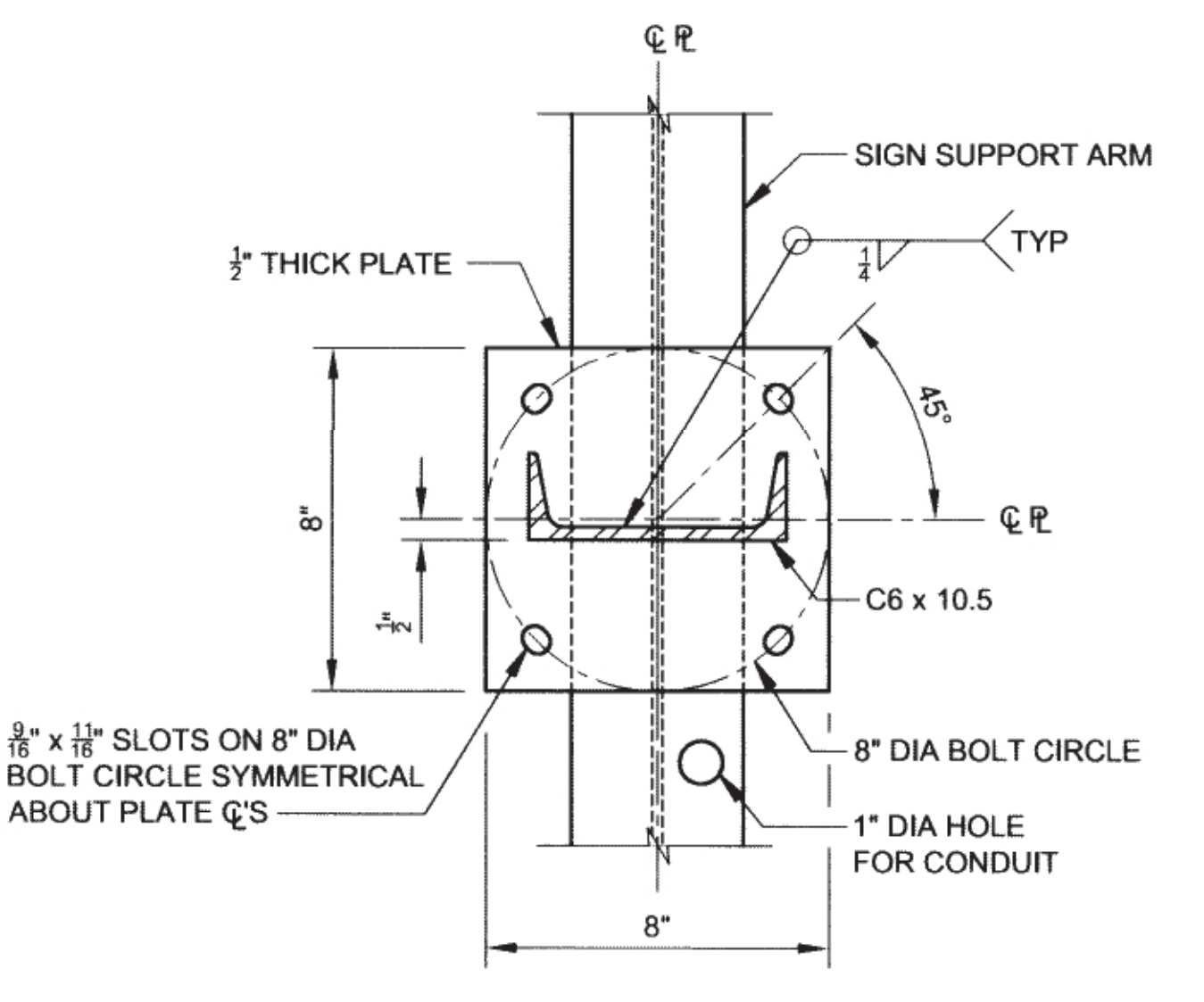
A9 SECTION F SCALE : 3" = 1'-0"
