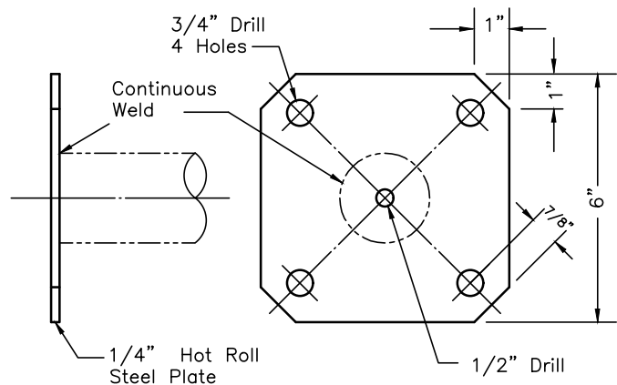
DETAIL: Post Flange Base
