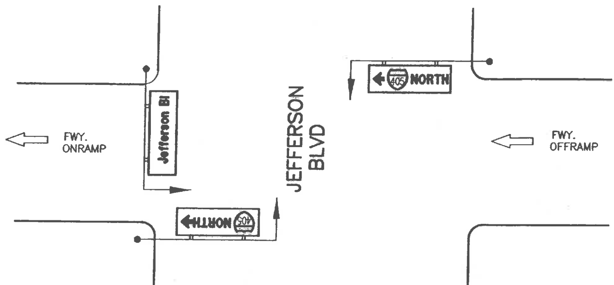
TYPICAL PLACEMENT
