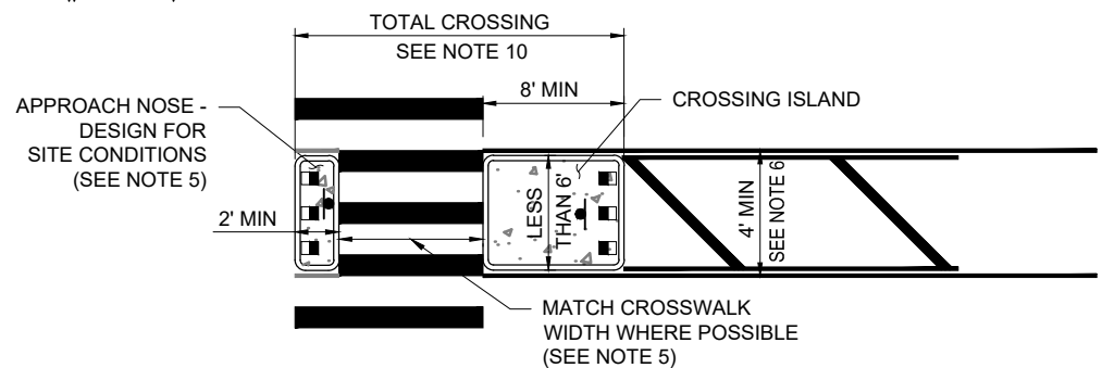
OPTION WHEN ISLAND IS LESS THAN 6' WIDE SEE NOTE 3
