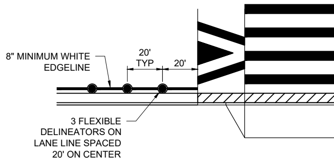
SIDEWALK CULVERT MARKINGS
